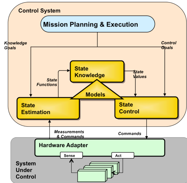
Figure 1 State-Based Control Architecture
