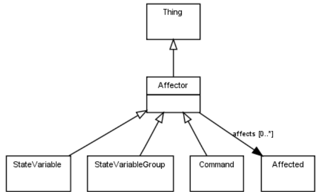
Figure 3 Affector Concept
