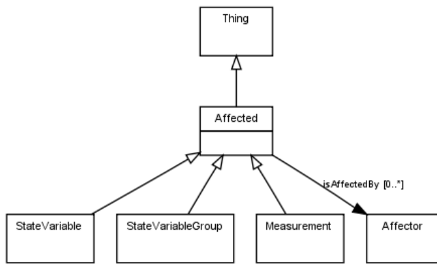
Figure 2 Affected Concept
