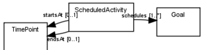
Figure 7 Goal Associations
