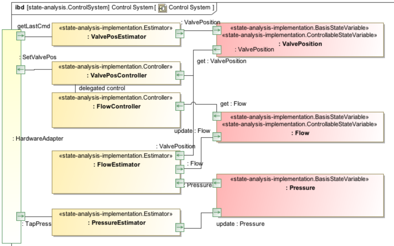
Figure 16 Functional Architecture
