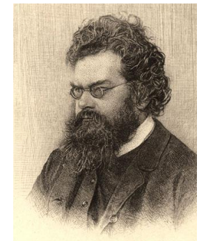
Boltzmann
