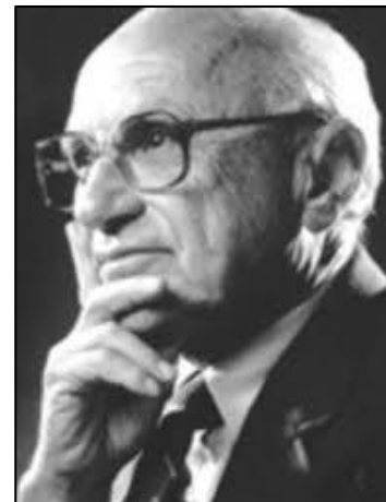
Friedman
