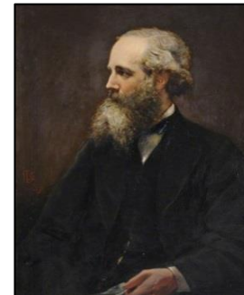
Maxwell
