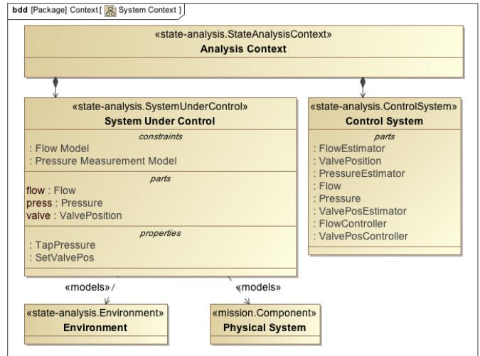
Figure 11 System Context Diagram
