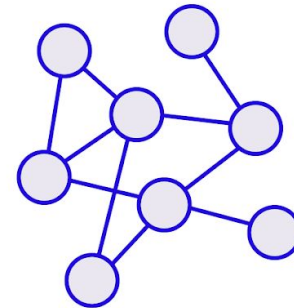
MICROSERVICES
